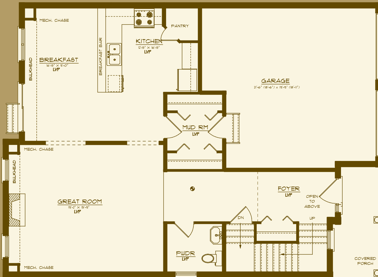
Main Floor 1,060 Sq. Ft.
